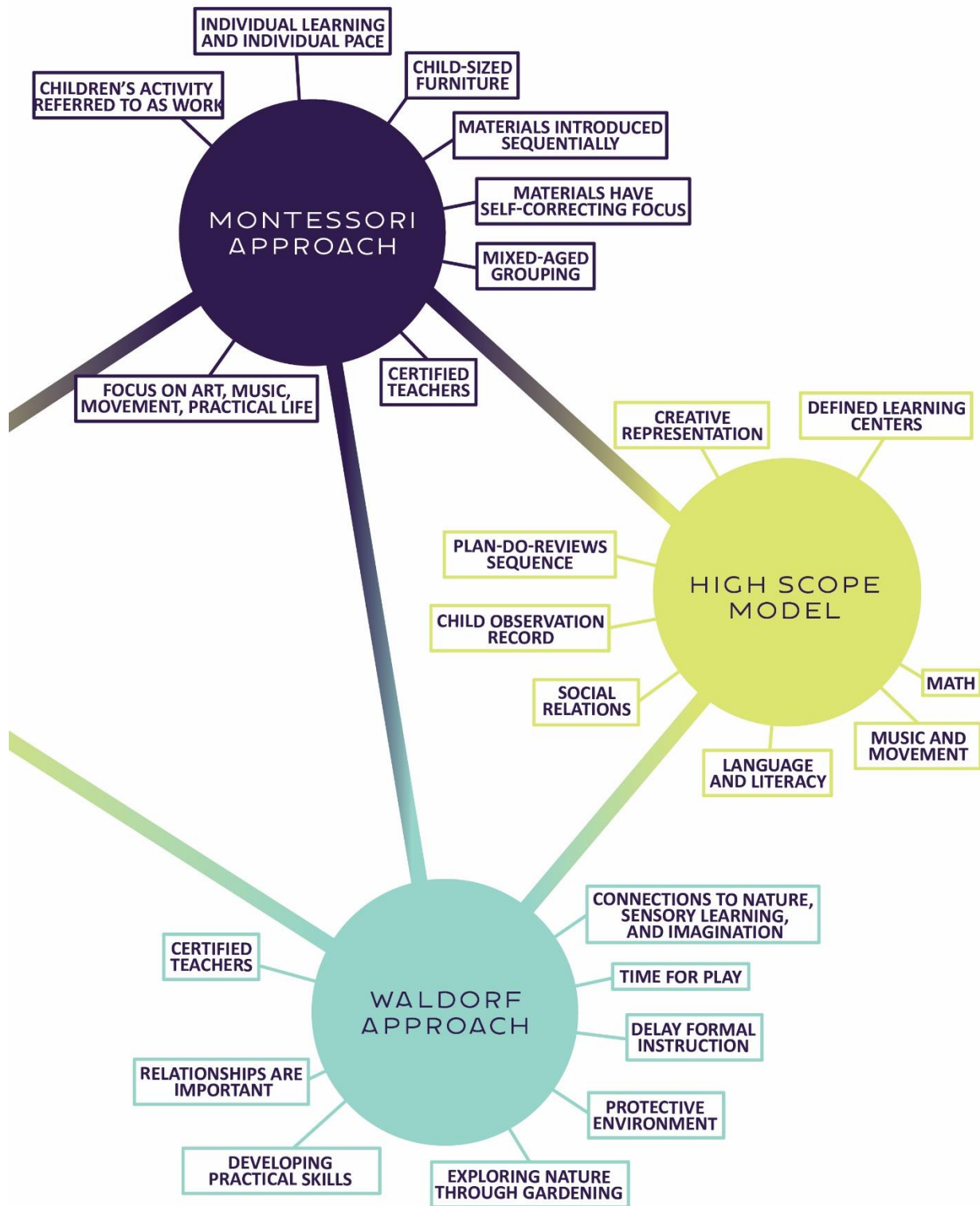
Figure 4.4: Curriculum models. 9
